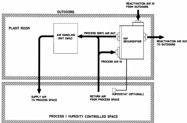
Installation with air handling unit
